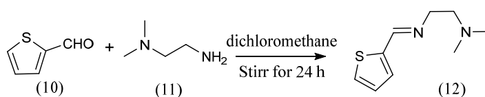
Scheme 4. Synthetic pathway by Jaegyong Lee et al. [31].
