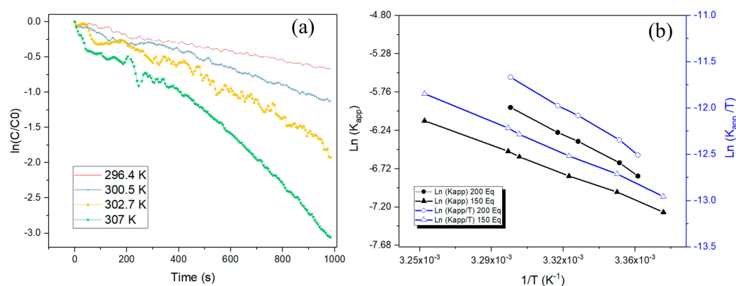
Figure 4. (a) \ln(C/C_0) versus time at different reaction temperatures, conditions of reaction 150 eq \text{BH}_4^- ; (b) Arrhenius plots \ln(k_{app}) and Eyring plots \ln(k_{app}/T) versus 1/T for the Pd nanoparticles.
