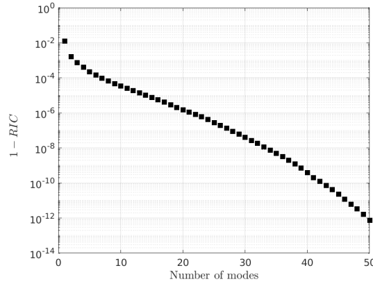
Figure 3. SVD: plot of k \mapsto 1 - \text{RIC}(k) , where \text{RIC}(k) represents the relative information content at truncation rank k .
