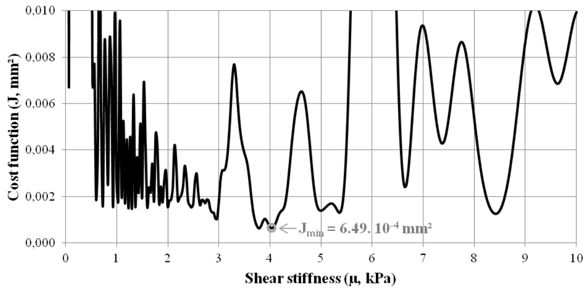
Fig. 4. Representation of the cost function ( J , \text{mm}^2 ) as a function of the shear stiffness ( \mu , \text{kPa} ), showing the result of the identification process.
