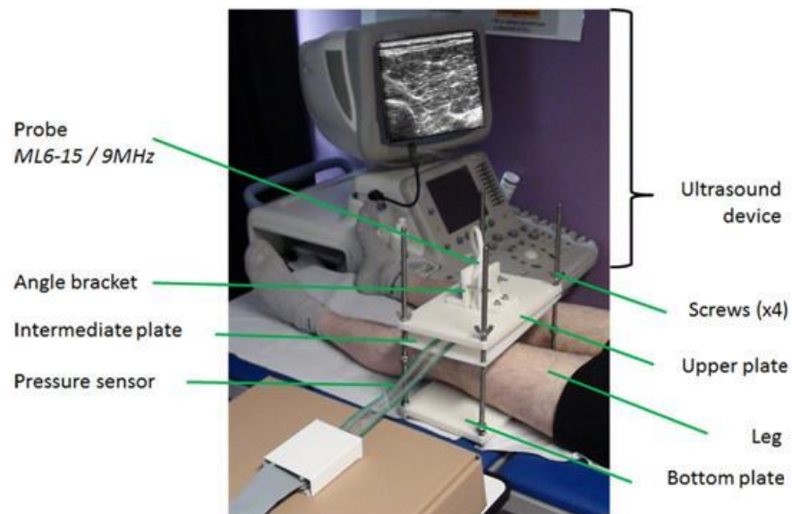
Fig. 2. Home-made compression device.
