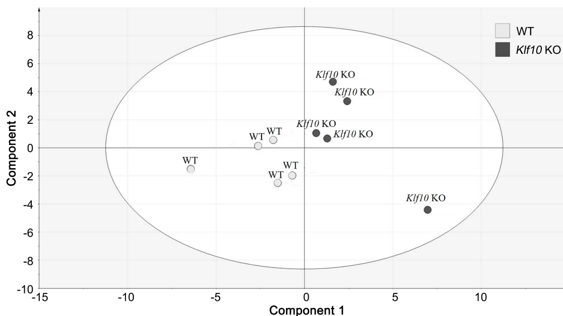
Figure 6. Partial Least Square Discriminant Analysis (PLS-DA) score resulting from modeling the 1 H-NMR spectral data matrix of WT (N = 5) and KO (N = 5) cerebellum, R 2 Y (cum) = 0.76, Q 2 = 0.7, X = 25. Klf10 KO: knockout Krüppel-like factor 10. WT: wild type.
