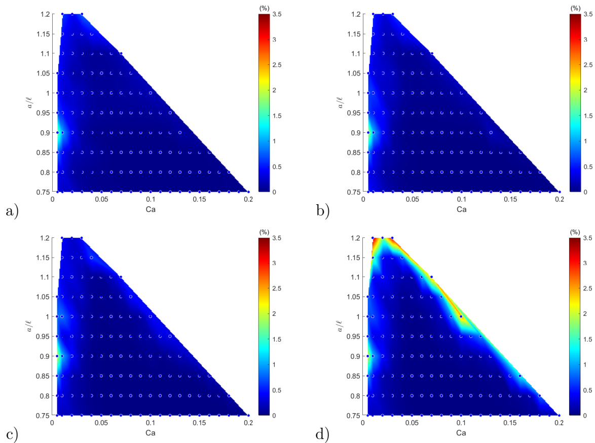
Figure 13. Heat maps of the normalized Hausdorff Distance d_{MH}/a of configuration prediction shapes over the parametric space at different transient states: (a) \gamma t = 1 ; (b) \gamma t = 2 ; (c) \gamma t = 4 ; and (d) \gamma t = 8 . The maximum error is 3.26% in (d).
