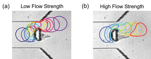
45 50 Fig. 7 Time-lapse images of soft capsules with D = 103 \mu\text{m} circumventing the half cylinder obstacle: (a) low flow strength; (b) high flow strength. The time interval between consecutive outlines is 20 ms at high flow strength, but variable at low flow strength. The duration of the sequence shown is 600 ms at low flow strength and 140 ms at high flow strength. The 55 elongated grey trail behind the obstacle is due to particles (e.g., small fragments of broken capsules) which are trapped in the stagnation region behind the obstacle.
