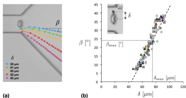
Fig. 2 (a) Trajectories of lycopodium particles with a diameter of approximately 20\ \mu\text{m} measured under high flow strength, for different values of the distance \delta between the particle centroid and the channel centreline, defined graphically in the inset of (b). (b) Variation of the trajectory angle \beta defined graphically in (a) as a function of \delta for lycopodium particles. Grey squares, triangles and diamonds correspond, respectively, to P_{\text{in}} = 267, 1200, 2400\ \text{mbar} and P_{\text{ext}} = 1000, 4500, 6000\ \text{mbar} . The coloured markers indicate the values of \beta associated with the trajectories shown in (a). The dashed line is a linear fit to the data. \delta_{\text{max}} = 75\ \mu\text{m} is the distance from the centreline of the channel to the middle of the constricted channel adjacent to the half-cylinder obstacle. The angle \beta_{\text{max}} = 24^\circ is the trajectory angle associated with \delta_{\text{max}} .
