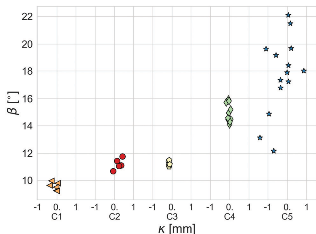
Fig. 5 Trajectory angle \beta from individual experiments plotted as a function of the offset \kappa for each capsule shown in Fig. 2 for Q = 10 ml min -1 . The initial offset of the capsules is |\kappa| \leq 0.5 mm ( |\kappa|/D \leq 0.13 ) and |\kappa| \leq 1.2 mm ( |\kappa|/D \leq 0.3 ) for the elastic bead C5.
