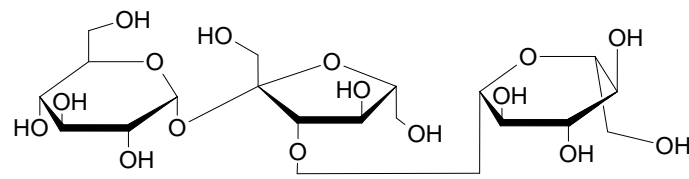
Figure 4. Melecitose structure.
