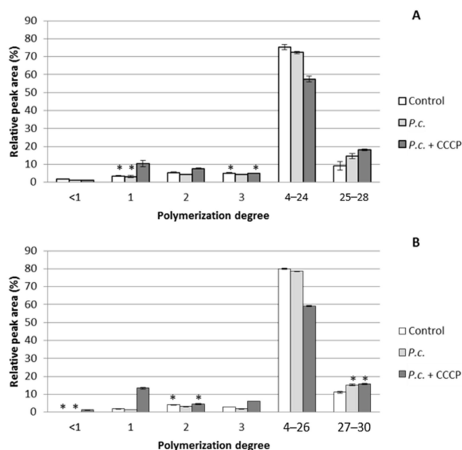
Figure 4. Impact of P. chrysosporium ( P.c. ) with and without CCCP on the polymerization degree of Kraft (A) and Organosolv (B) lignins after 11 days of incubation in a mineral medium at pH 5.5 and a C/N ratio of 21.34 (asterisks indicate averages that were not statistically different according to an unpaired Student t -test at a 99% confidence level for the same polymerization degree).
