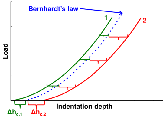
Figure 1 Schematic drawing of the meaning of \Delta h_c , the error between the shape of the loading curves predicted by Bernhardt's law and the shape of the experimental curves.
