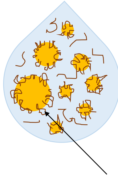
Emulsion drop
