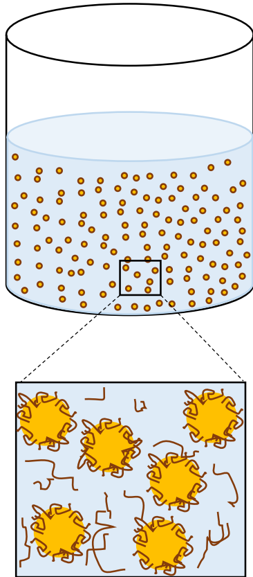
O/W emulsion
