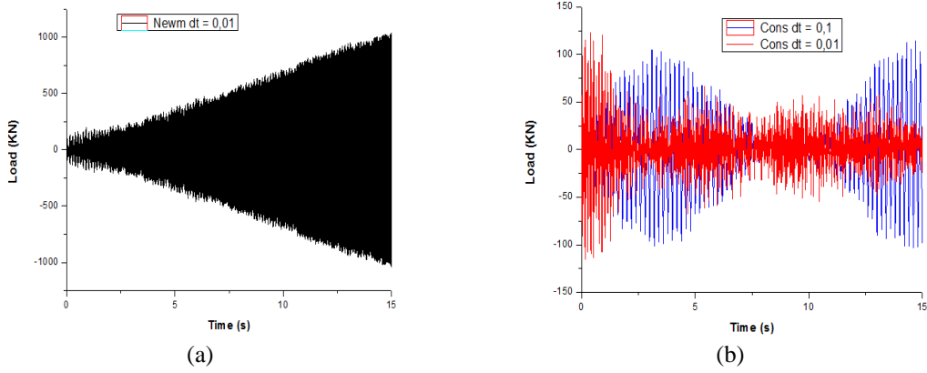
Fig. 25 Force versus Time computed by Newmark scheme (a) and energy-conserving scheme (b)
