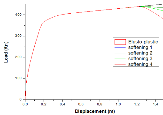
Fig. 19 Response of six story frame using different softening's modulus
