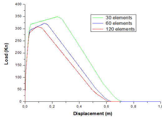
Fig. 15 Response of the frame up to the total collapse using different mesh
