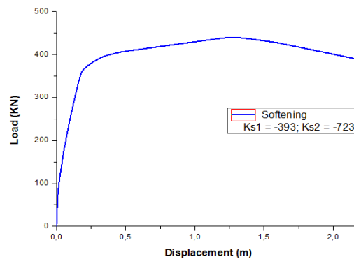
Fig. 20 Response of six-story frame up to the creation of all plastic hinges
