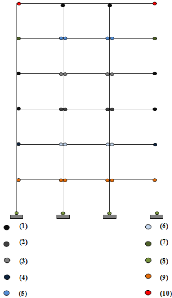
Fig. 21 Location of softening plastic hinges in six-story frame
