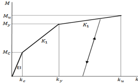
Fig. 2 Moment-curvature relation for bending stress resultant model
