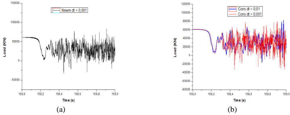
Fig. 27 Force versus Time computed by Newmark scheme (a) and energy-conserving scheme (b): structure in contact with ground
