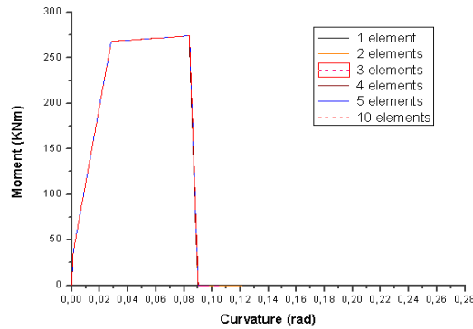
Fig. 9 Cantilever beam with end moment: Different number of elements with one weakened
