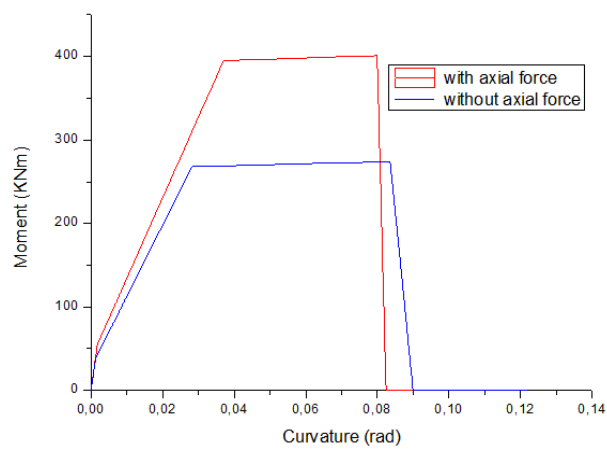
Fig. 11 Cantilever beam response under end moment with and without axial force
