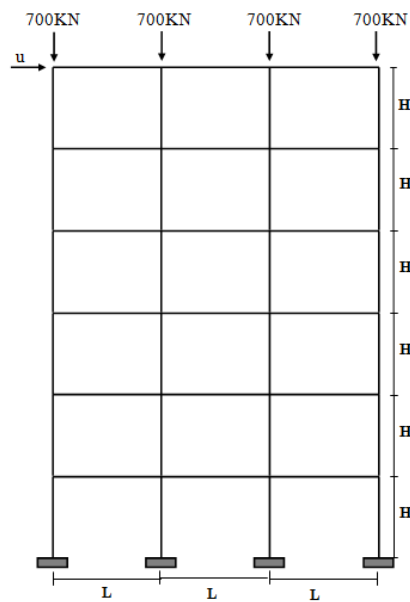
Fig. 17 Six story frame
