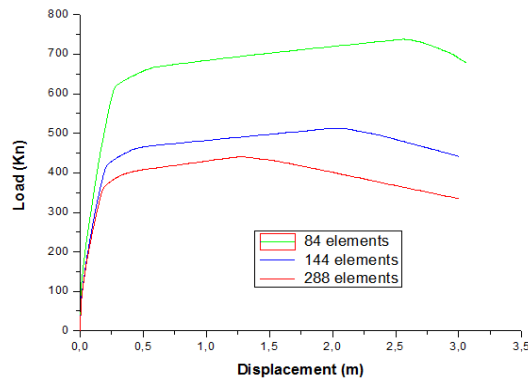
Fig. 18 Response of six story frame using different mesh
