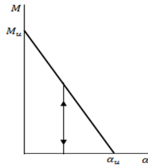
Fig. 4 Moment-jump relation for softening
